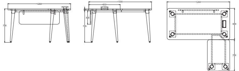
L Shape Desk (1)
