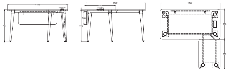
L Shape Desk (2)
