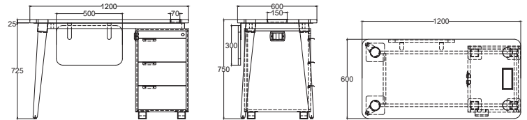
Desk with Drawer (1)
