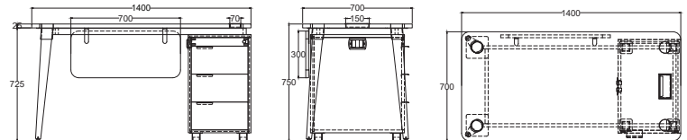
Desk with Drawer (2)
